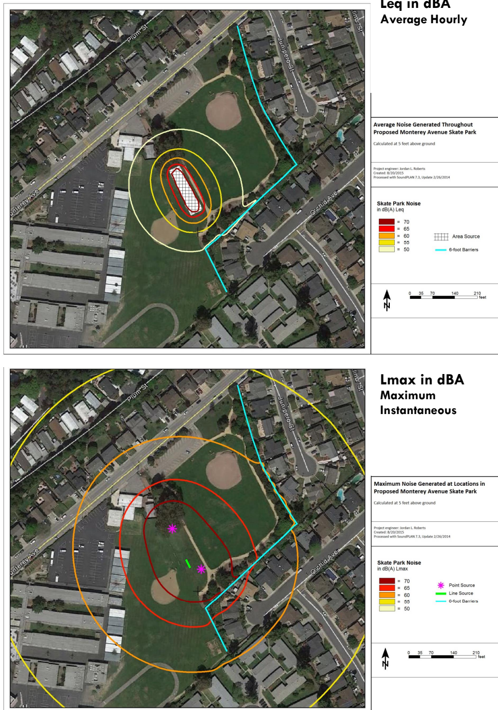
FIGURE 4.3-2: Noise Generated by Proposed Skate Park
