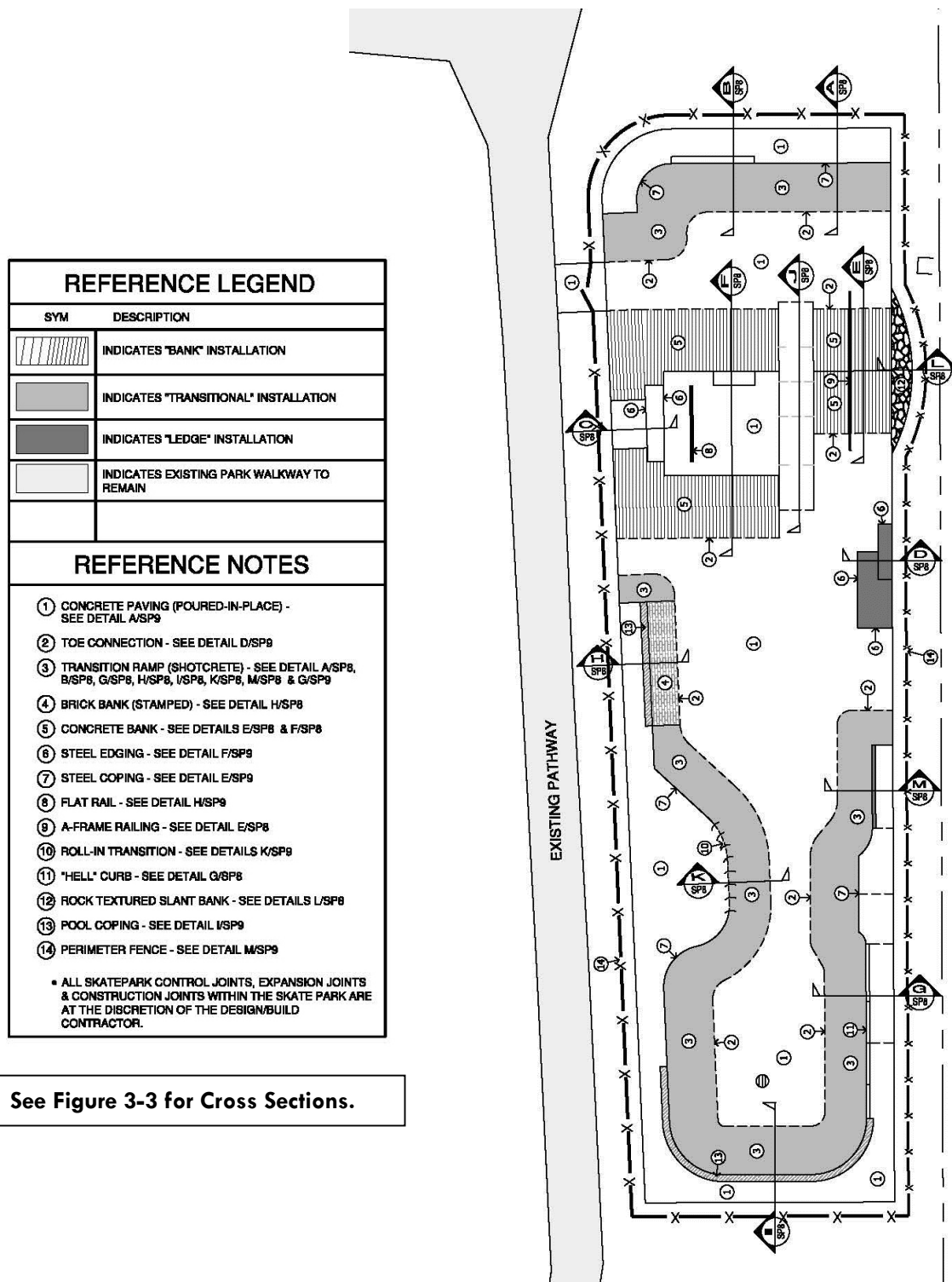
FIGURE 2-2: Proposed Skate Park Features
