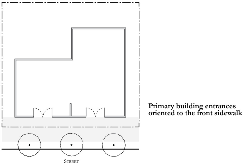
FIGURE 17.20-2: BUILDING ORIENTATION
